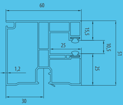
Rail de guidage standard PVC
